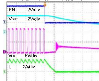
Shutdown
